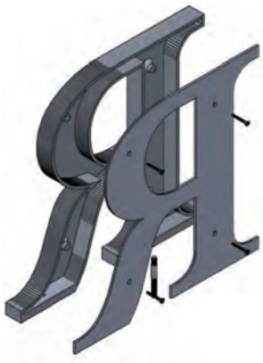
Bottom Stud w/Back Cover Multiply the brushed letter price by 2 Letters 4"-24", Minimum 3/8" thick Includes painted or anodized 1/8" thick aluminum back. Letters over 8" may require tie-back (not supplied). Can be full cover or inset for flush edge.
